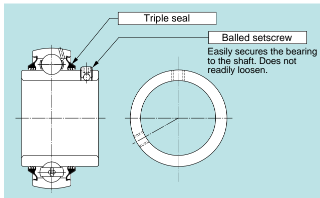
Triple-sealed bearing
